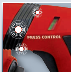
Vibration absorption with press control
