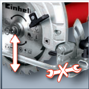
Toolless cutting depth adjustment
