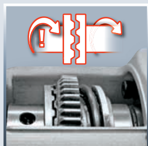
Safety slip coupling
